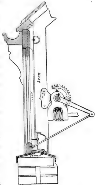
FIG. 17. IRON POST AND SILL, WITH SIDE VENTILATION.
